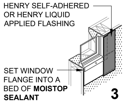
WINDOW FLASHING ISOMETRIC VIEW
