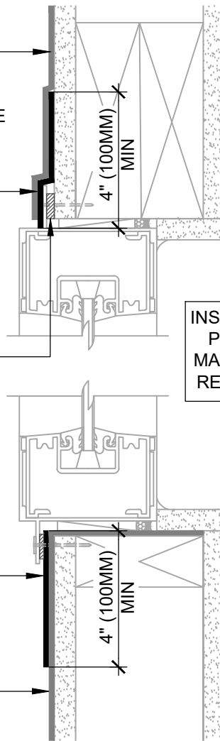
ASTM E2112 - METHOD A1 SECTION VIEW
