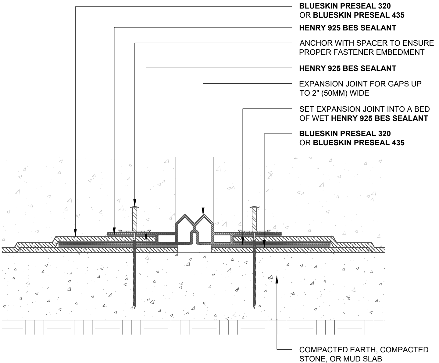
SECTION VIEW DECK TO DECK
