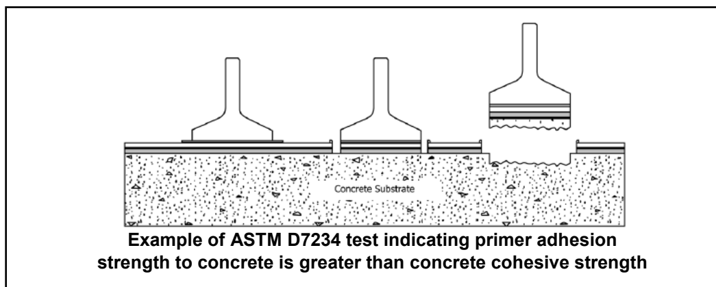
Source: Figure 2 excerpt from ASTM D7234 – Standard Test Method for Pull-Off Adhesion Strength of Coatings on Concrete Using Portable Pull-Off Adhesion Testers
