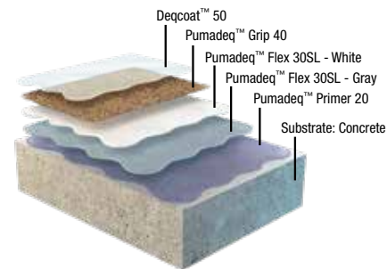
Vehicular Traffic System
