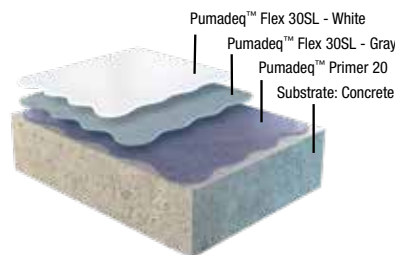
Plaza Deck System (typical unreinforced system)
