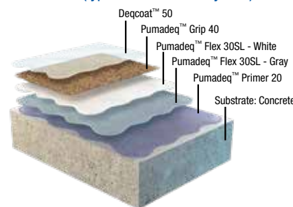
Pedestrian / Balcony System (typical unreinforced system)
