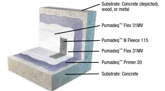
Flashing System
